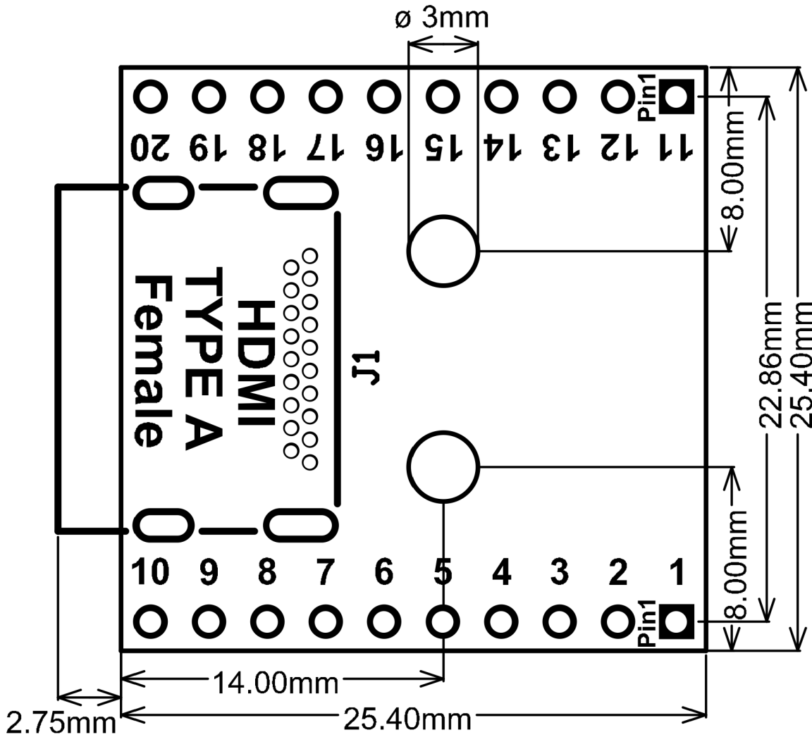
HDMI-AF-BO-V1A PCB outline Drawing
