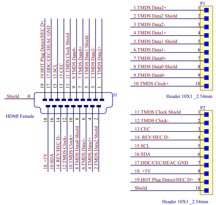
HDMI-AF-BO-V1A Schematic Diagram
